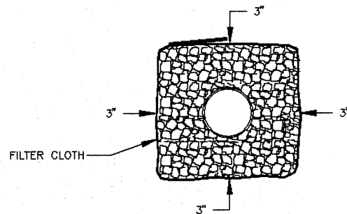
Figure C-11 Subsurface Drain Envelope Schematic
