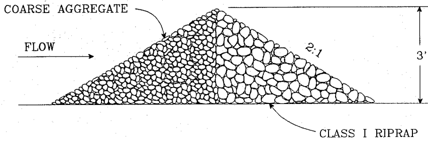
Figure C-21 Schematic Diagram of a Rock Check Dam
