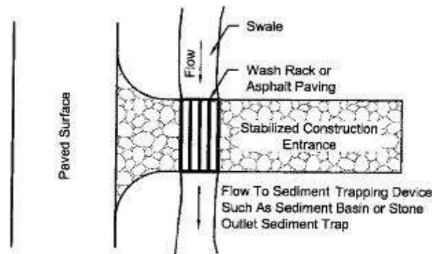
Figure C-17 Schematic Tire Wash Facility
