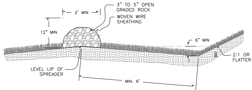
LEVEL SPREADER WITH ROCK BERM LIP
