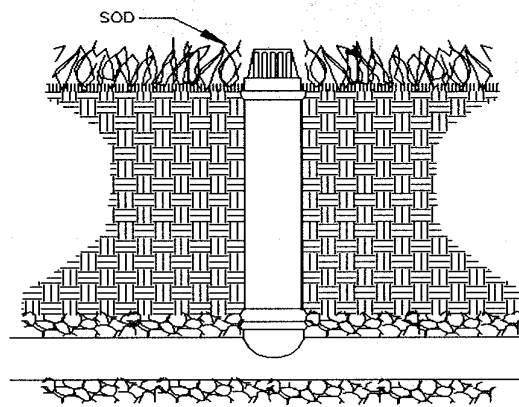
GRATED INLET
