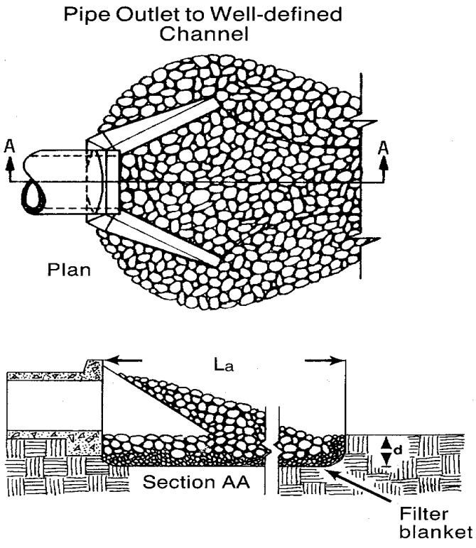
Figure C-5 Schematic Riprap Outlet Design
