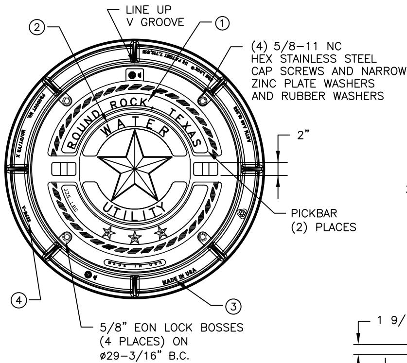
COVER PLAN VIEW
