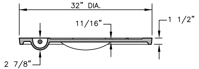
COVER SECTION VIEW
