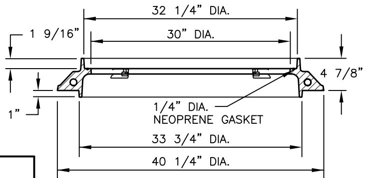
FRAME SECTION VIEW
