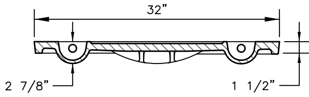
MANHOLE COVER SECTION VIEW
