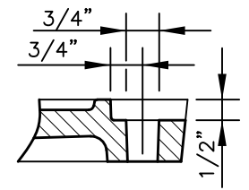
BOLT HOLE SECTION
