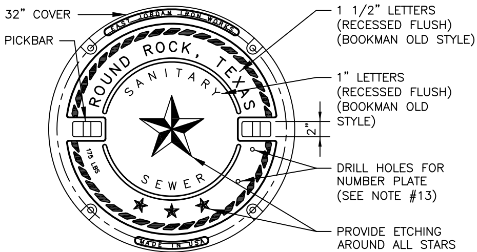
MANHOLE COVER PLAN VIEW
