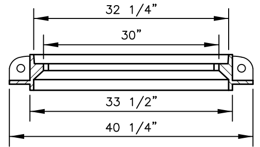
MANHOLE FRAME SECTION VIEW
