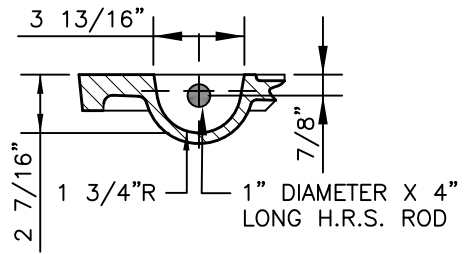
PICKBAR DETAIL
