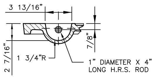
PICKBAR DETAIL
