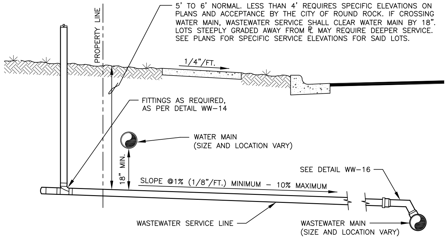
SECTION "A-A"
