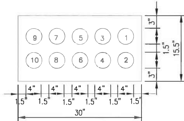
TYPICAL 4" COMMUNICATIONS LAYOUT NTS
