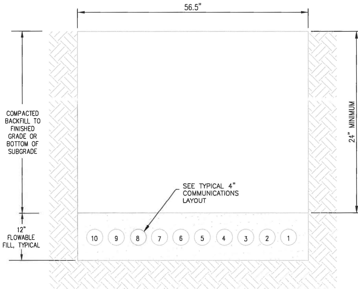
DUCT BANK LINE DETAIL NTS
