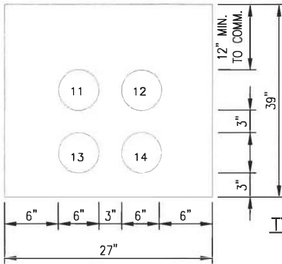
TYPICAL 6" ELECTRICAL LAYOUT NTS
