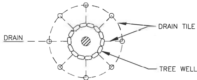
TREE WELL WITH RAISED GRADE
