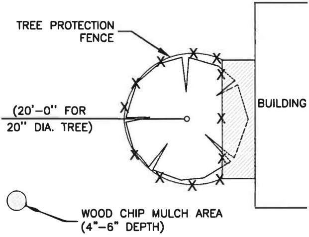
TREE PROTECTION FENCE (MODIFIED) – CHAIN LINK
