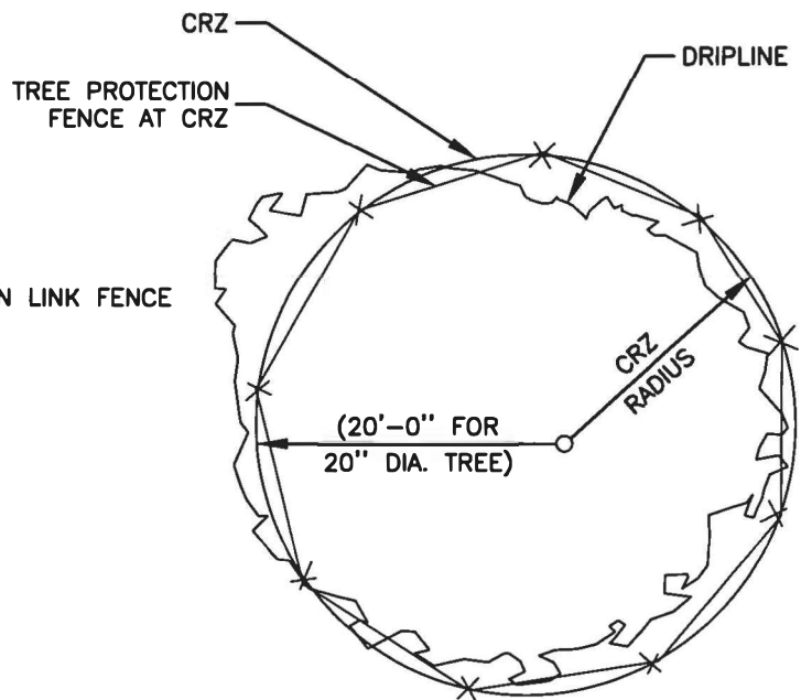
TREE PROTECTION FENCE – CHAIN LINK
