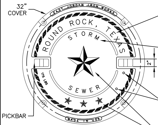
MANHOLE COVER PLAN VIEW
