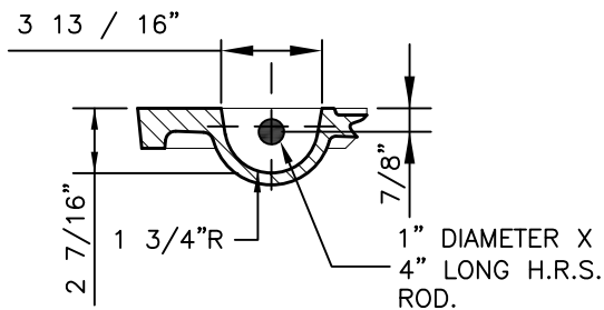
PICKBAR DETAIL
