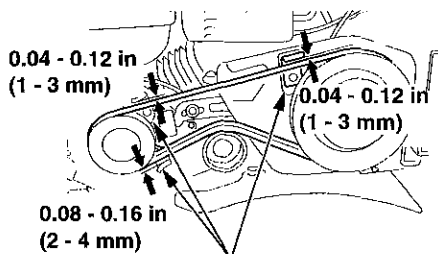
BELT STOPPER
