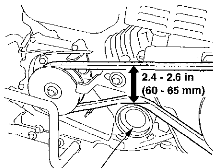
TENSION ROLLER
