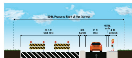
Traffic Control During Construction
